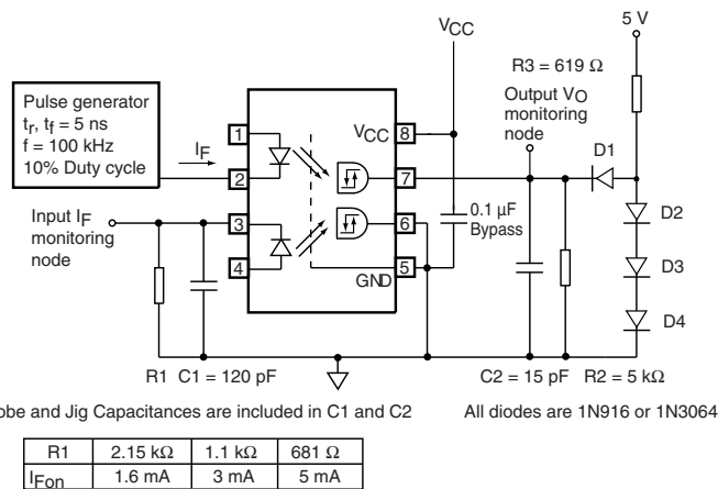
Fig. 19 - Test Circuit for t_{PLH}
