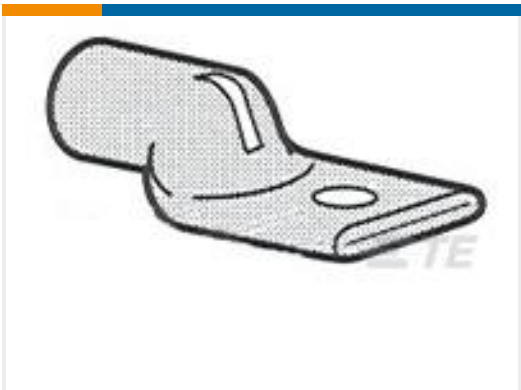
TE Part #325603-2 TERMINAL,AMPOWER 4/0
