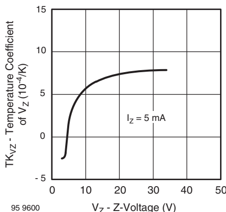
Fig. 5 - Temperature Coefficient of V_Z vs. Z-Voltage
