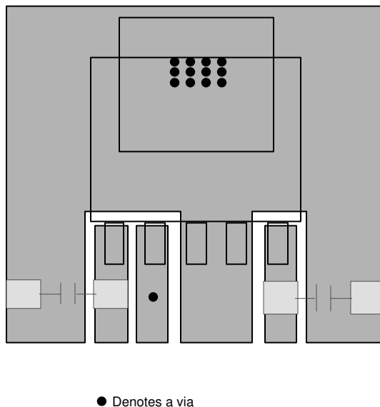
Figure 8-12. KVV Package Fixed Output
