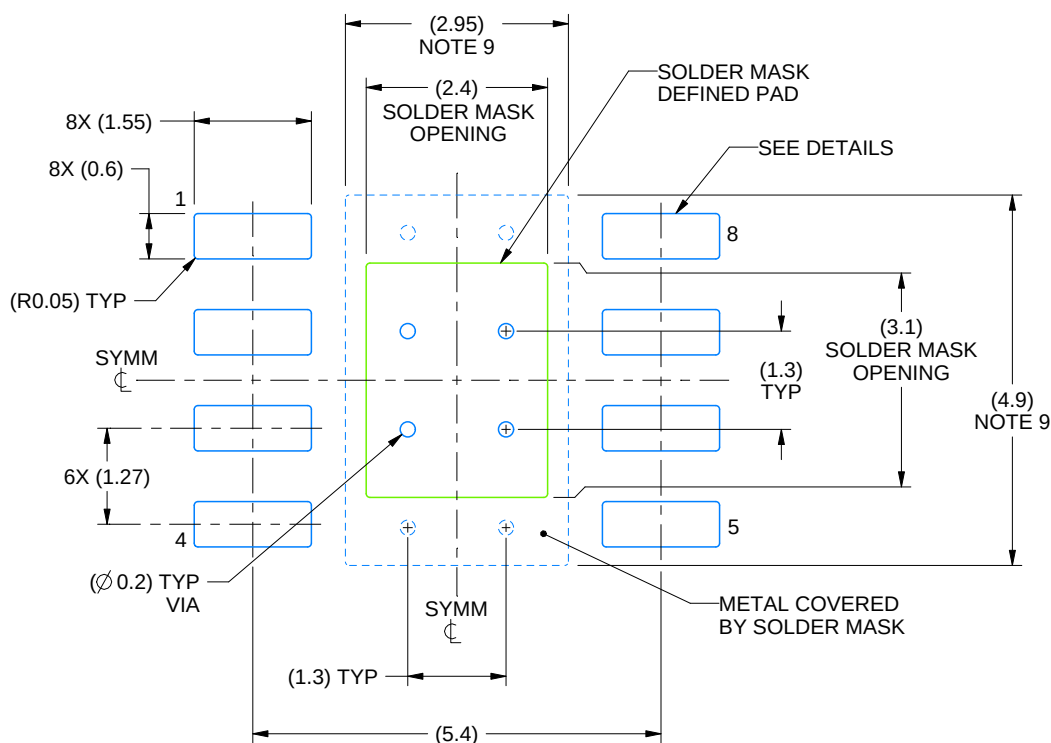
LAND PATTERN EXAMPLE EXPOSED METAL SHOWN SCALE:10X
