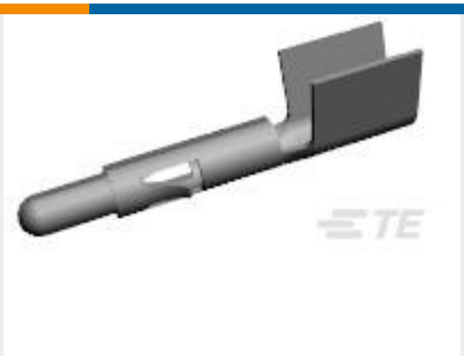
TE Part #640309-6 UMNL PIN 12-10 AU/PHBZ
