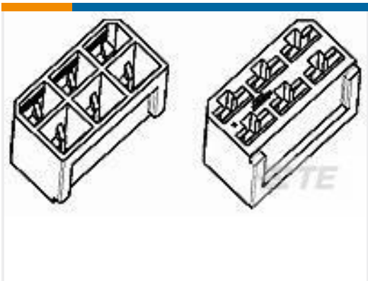
TE Part #280314 FF 250 REC HSG 6P NYLON CLEAR
