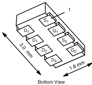
1206-8 Chip (Dual)
