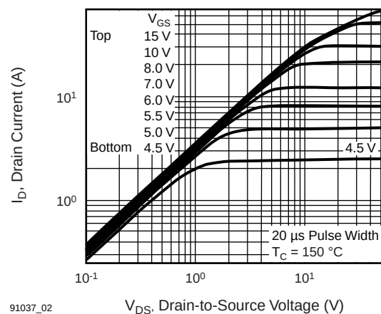
Fig. 2 - Typical Output Characteristics, T_J = 175^\circ\text{C}
