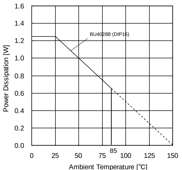
Figure 8. Derating Curve
