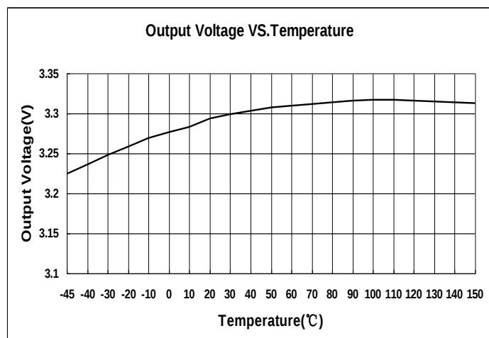
(5) Output Voltage VS. Temperature (ME6209A33PG)
