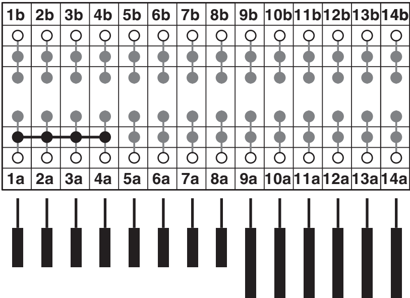
Circuit diagram
