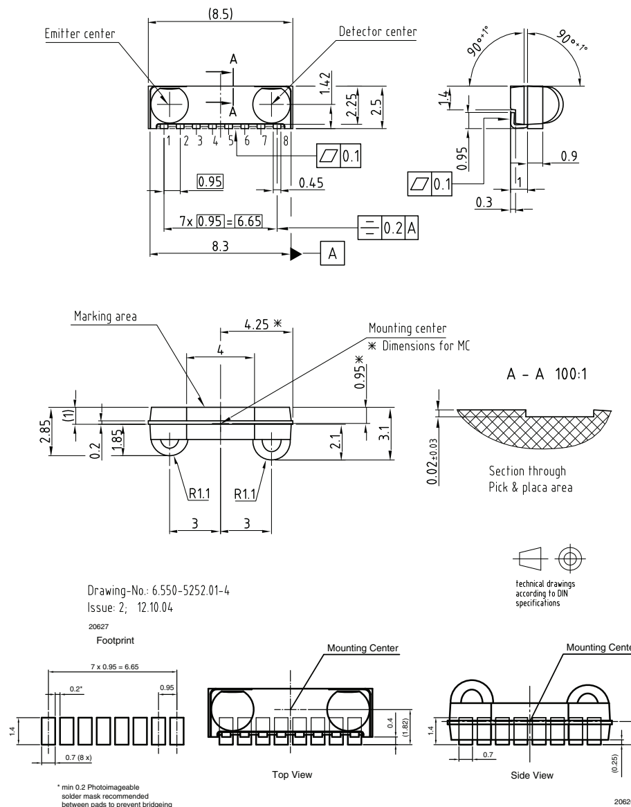
Fig. 8 - Package Drawing
