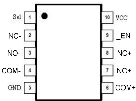
MSOP-10
