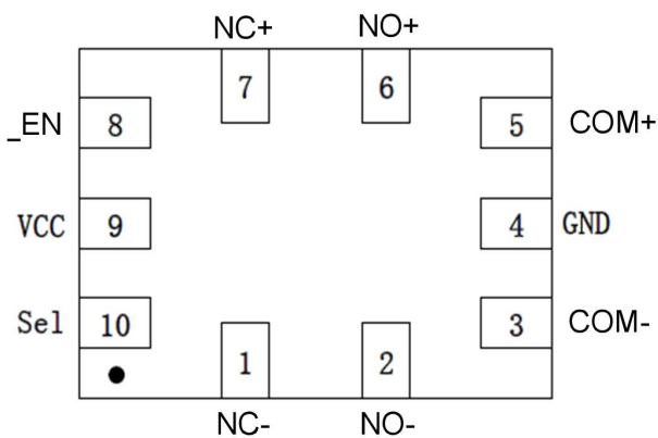
QFN1418
