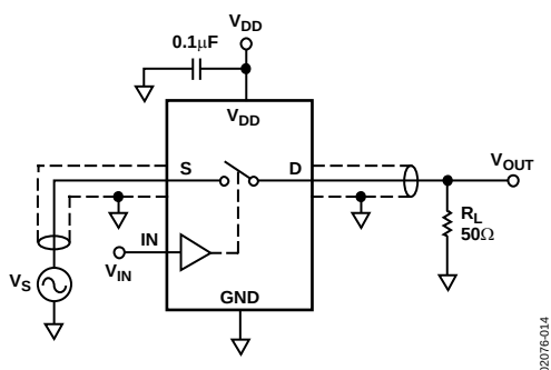
Figure 16. Off Isolation
