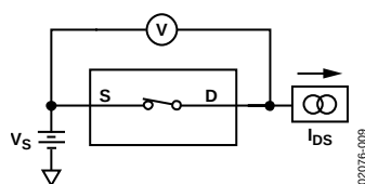
Figure 11. On Resistance
