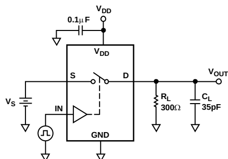
Figure 14. Switching Times
