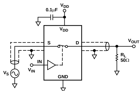
Figure 17. Bandwidth
