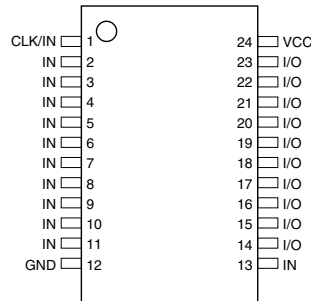
Figure 2-1. TSSOP
