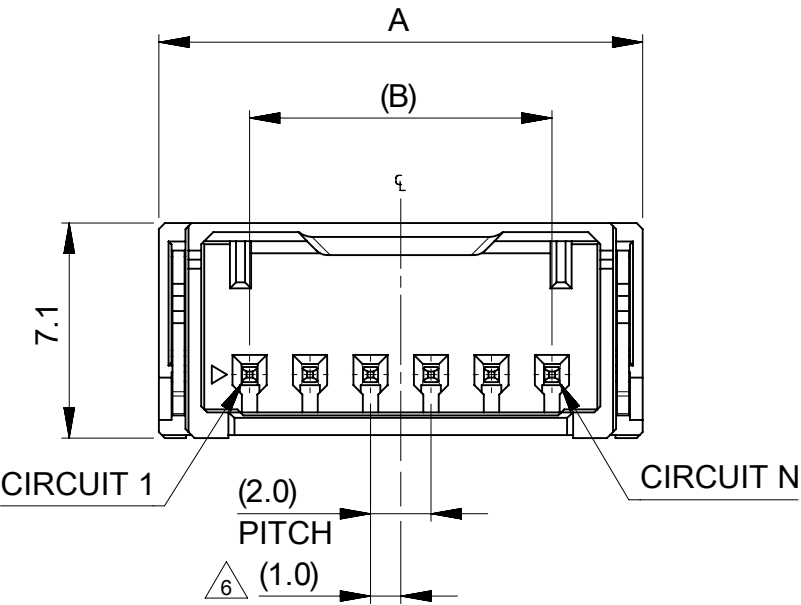
VIEW OF 2-3 CIRCUIT
