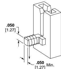
Wrap Post Part Number 1601447
