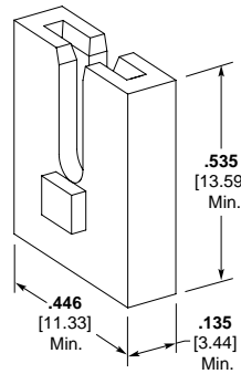
Cavity Part Number 1601435
