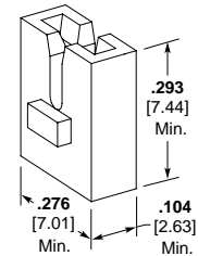
Cavity Part Number 1601434
