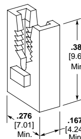
Cavity Part Number 1601463
