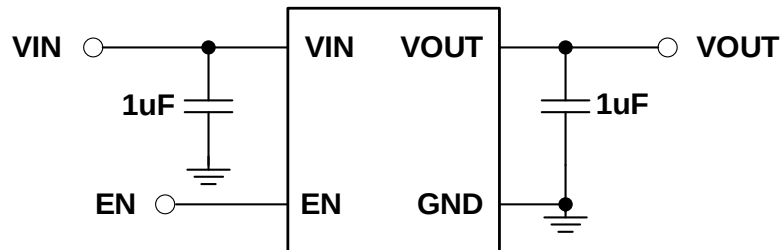
Figure 2(A), Typical Application Schematics of OCP2820VxxAD & OCP2820WExxAD
