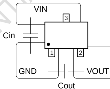
Figure 4(B), Recommended PCB Layout of OCP2820WxxAD
