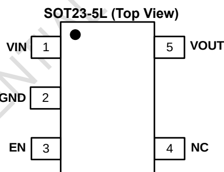
Figure 1(C), Pin Assignments of OCP2820WExxAD
