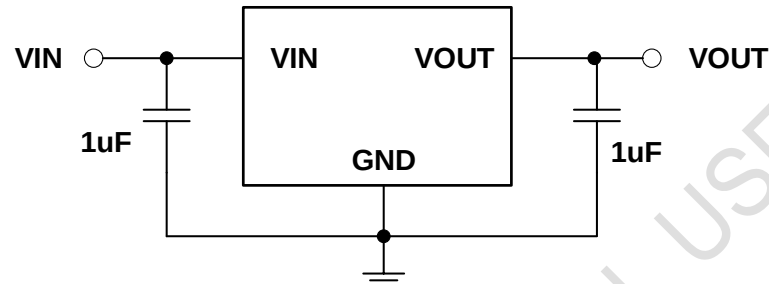
Figure 2(B), Typical Application Schematics of OCP2820WxxAD
