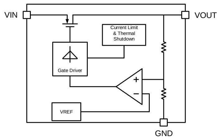
Figure 3(B), Typical Application Block diagram of OCP2820WxxAD
