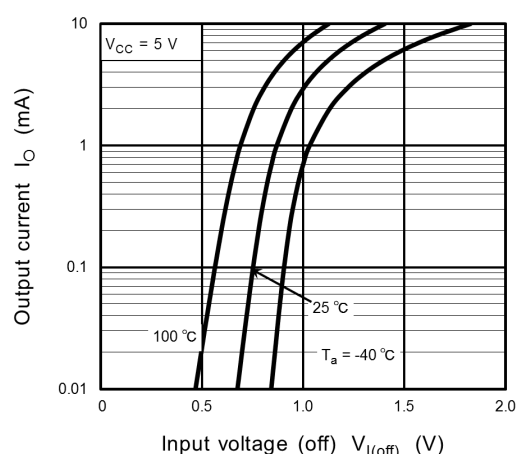
Fig. 7.2 I_O - V_{I(off)}
