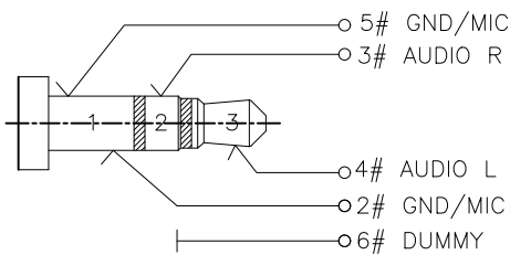
SCHEMATIC
