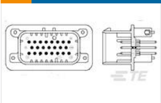
TE Part #776231-4 35POS,PIN DIA 1.3,HDR ASSY, 180DEG,COD 4
