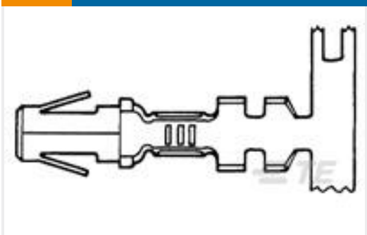
TE Part #350200-1 .140 DIA SOK 14-10 PTPBR
