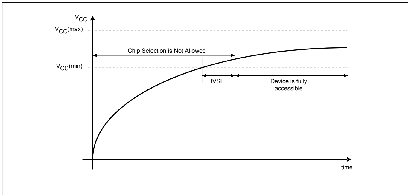
Figure 27. Power-up Timing
