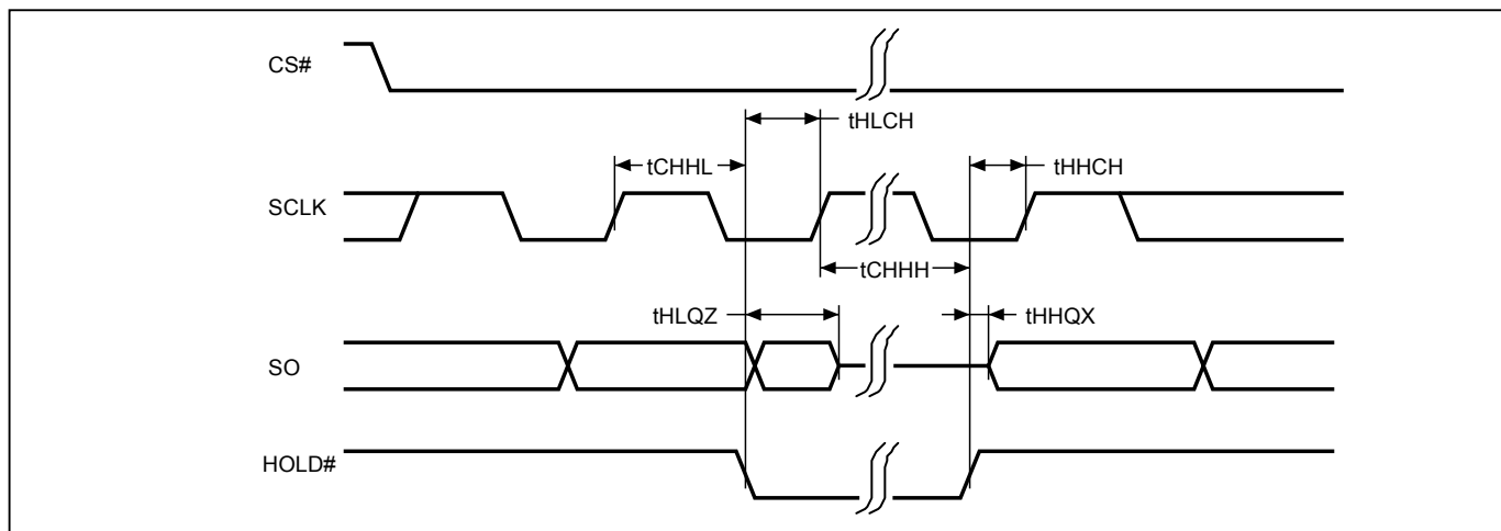
Figure 9. Hold Timing
