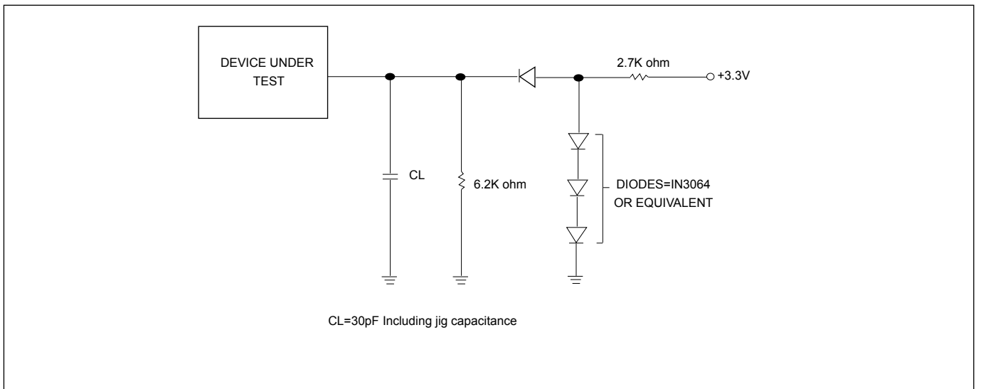
Figure 6. OUTPUT LOADING
