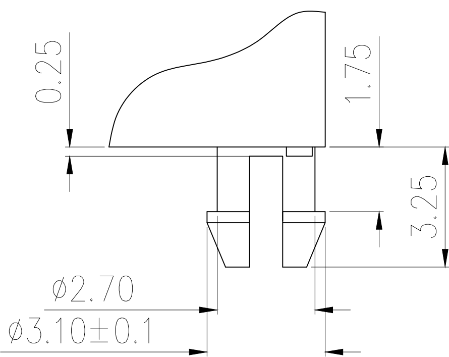
DETAIL "X" SCALE 2:1
