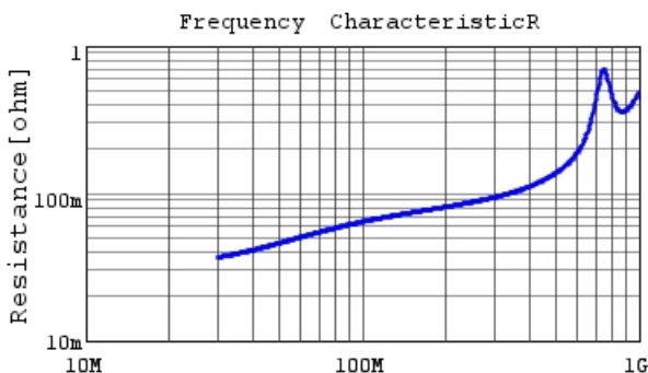
RCE5C2J471J1M1H03A R DCOV, 25degC
