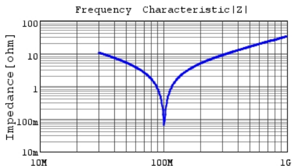
RCE5C2J471J1M1H03A |Z| DCOV, 25degC
