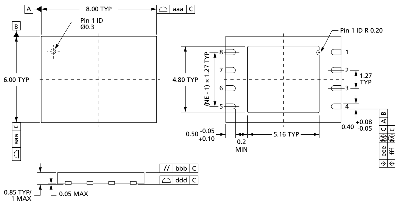
Figure 41: V-PDFN-8 8mm x 6mm (MLP8) – Package Code: F8
