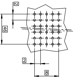
LAYOUT FOR P.C.B
