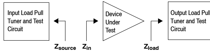
Figure 8. Load Pull Performance — Maximum P1dB Tuning
