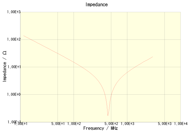
C3216C0G2J101J060AA
