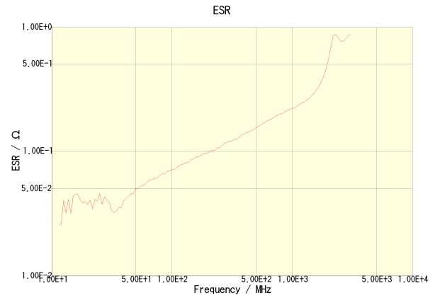
C3216C0G2J101J060AA
