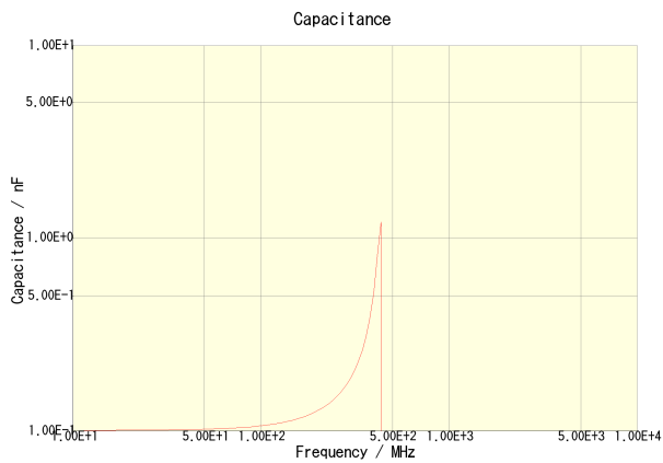
C3216C0G2J101J060AA
