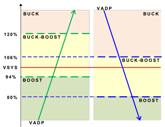
FIGURE 31. OPERATION MODE
