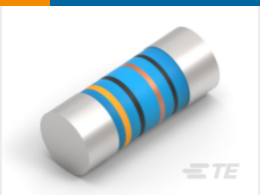
TE Part #7-2176314-8 MELF SMA-A 56R 1% 50PPM 0102 0.3 W
