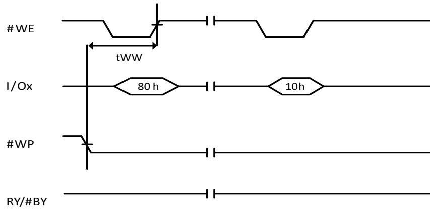
Figure 9-15 Program Disable
