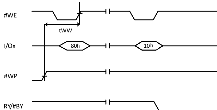
Figure 9-14 Program Enable
