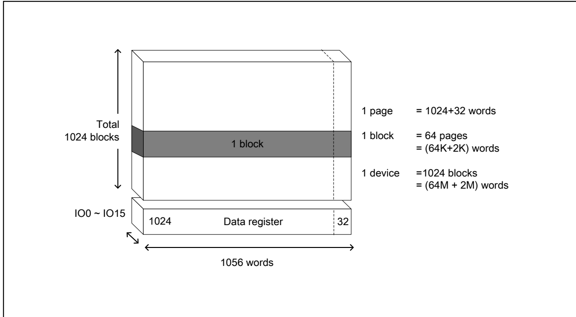
Figure 6-2 Array Organization
