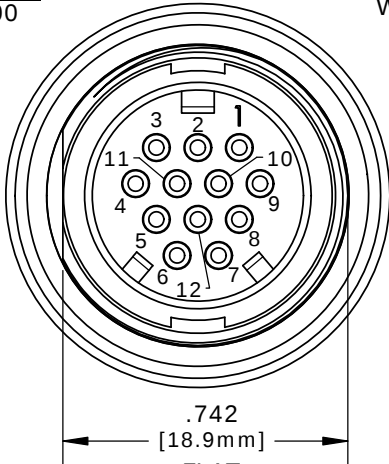
MATING VIEW W4292-12PG-300 12-POS.
