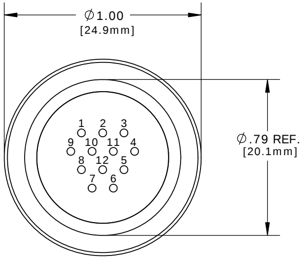
PC TAIL VIEW W4292-10PG-300 - 10-POS. (11&12 CLOSED) W4292-11PG-300 - 11-POS. (12 CLOSED) W4292-12PG-300 - 12-POS. (ALL OPEN)
