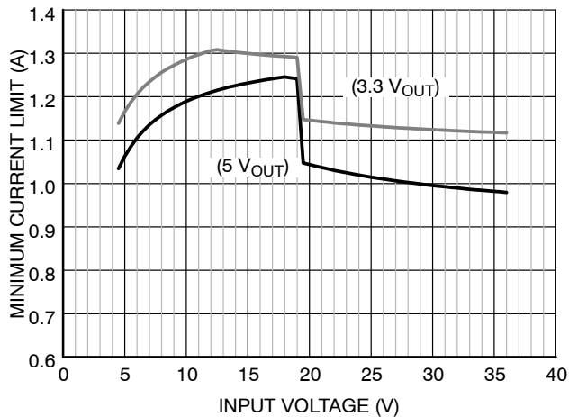
Figure 26. NCV890130 Load Current Capability with 4.7 \mu\text{H} Inductor
