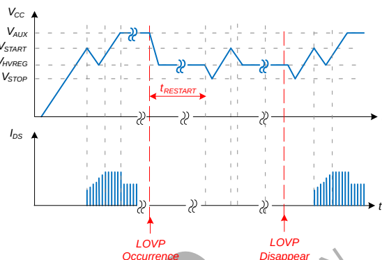
Figure 25. LOVP Waveforms
