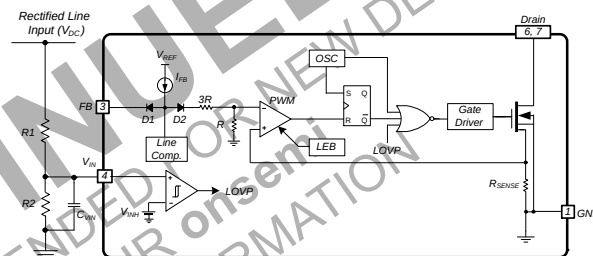
Figure 26. LOVP Circuit
