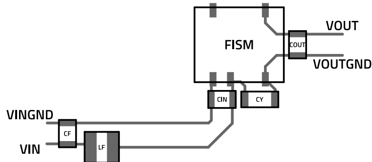
Figure 12: Layout recommendation.
