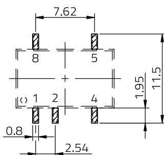
Figure 20: Recommended landpattern dimensions.
