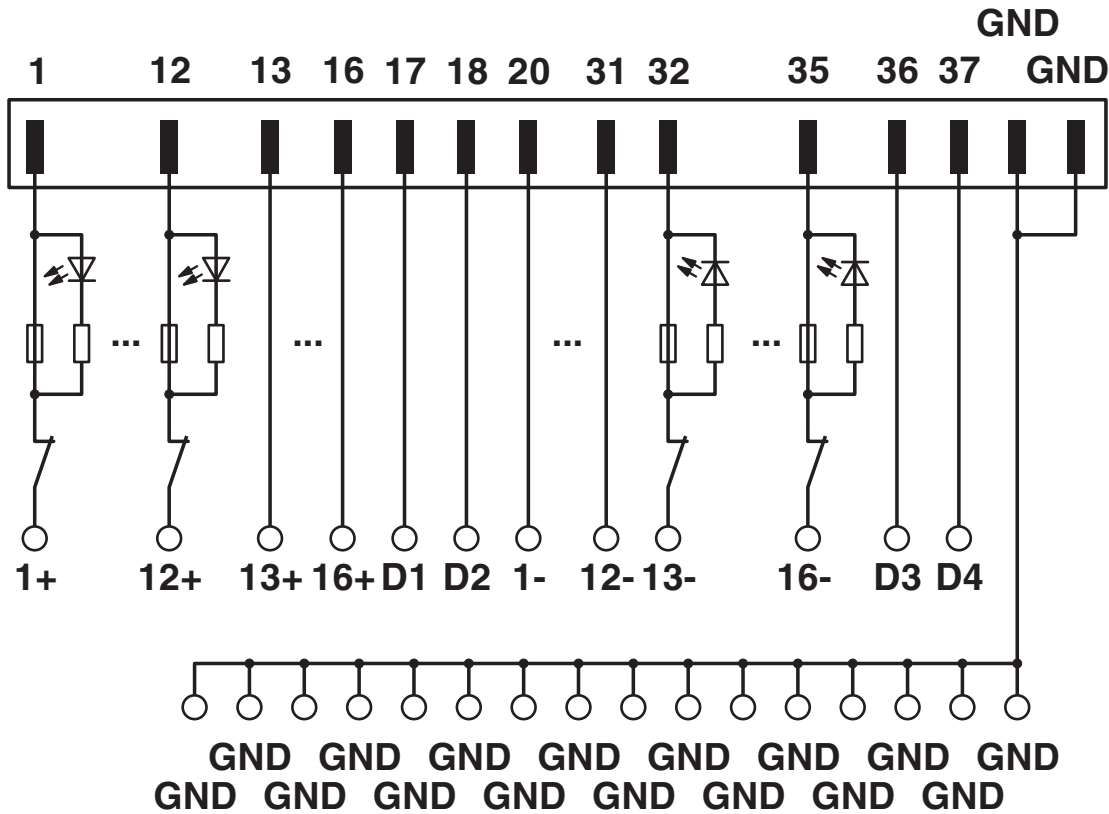
Circuit diagram
