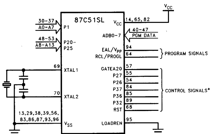
Figure 8. Programming/Verifying the OTP
