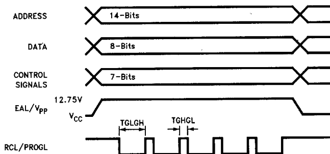
Figure 9. Programming Signal's Waveforms
