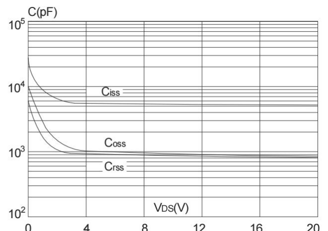
Capacitance Characteristics
