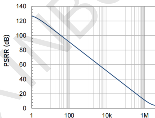
Frequency (Hz) Power Supply Rejection Ratio as a function of Frequency.
