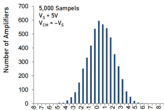
Input Offset Voltage ( \mu\text{V} ) Input Offset Voltage Production Distribution.
