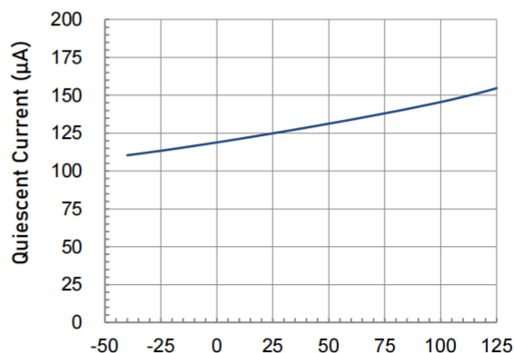
Temperature ( ^\circ\text{C} ) Quiescent Current as a function of Temperature.
