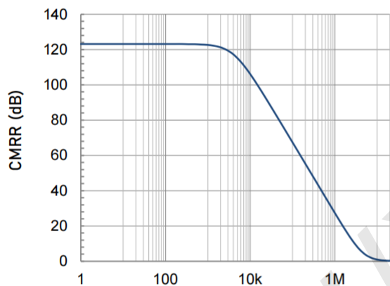
Frequency (Hz) Common-mode Rejection Ratio as a function of Frequency.
