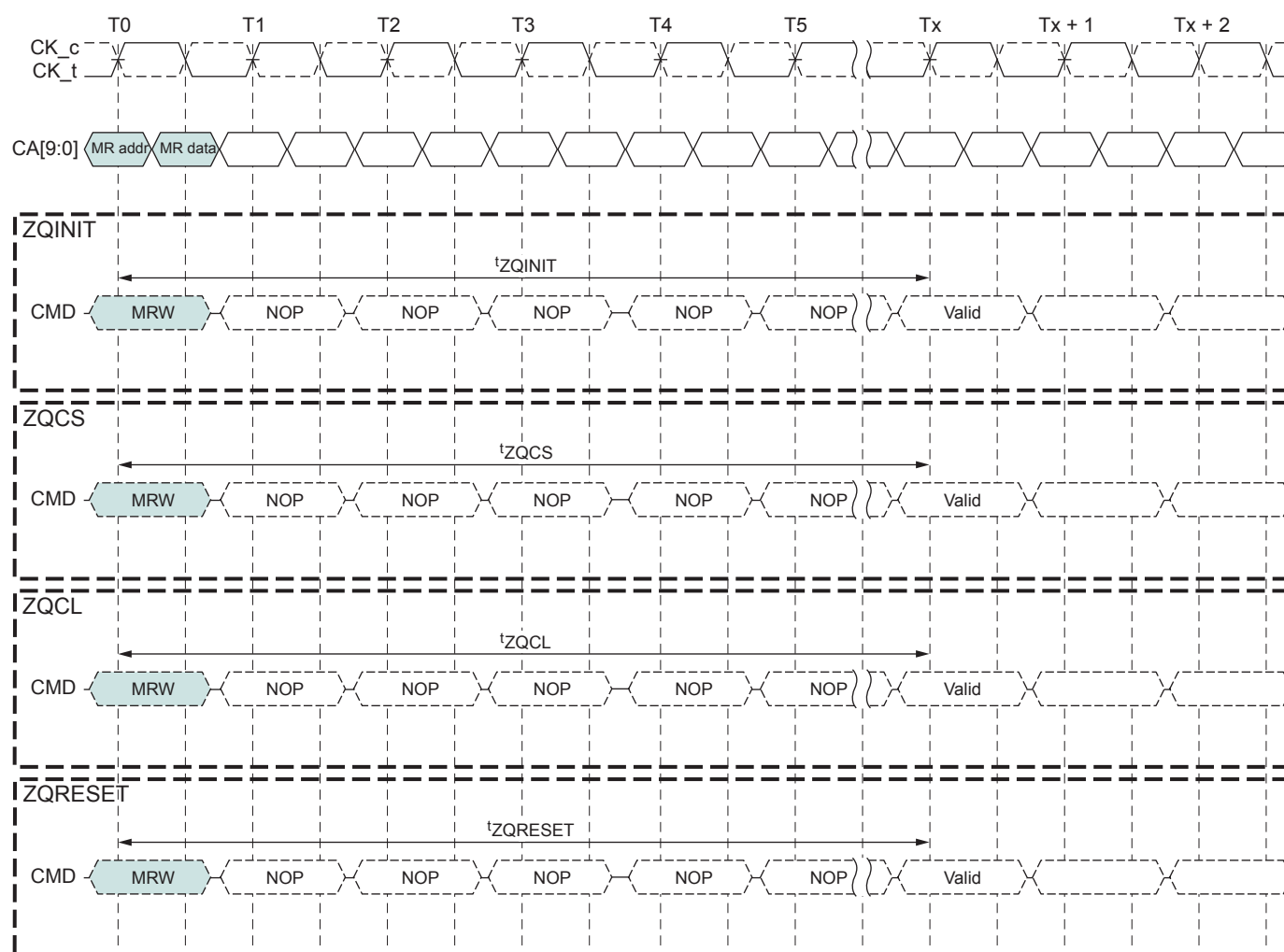
Figure 55: ZQ Timings
