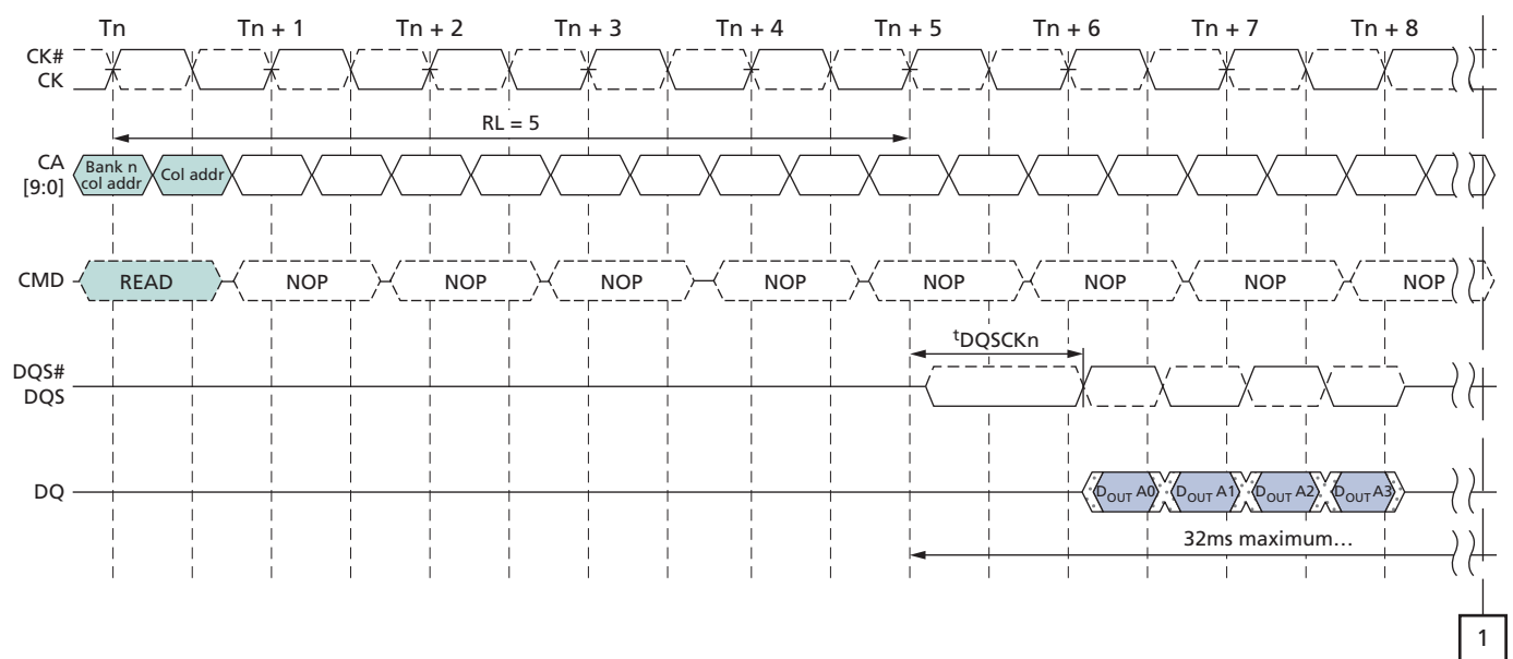
Figure 21: t_{DQSKDL} Timing
