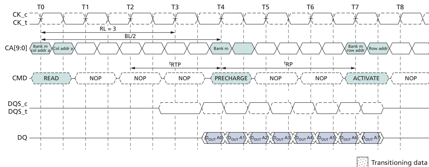
Figure 36: READ Burst Followed by PRECHARGE – RL = 3, BL = 8, RU(t_{RTP}(\text{MIN})/t_{CK}) = 2
