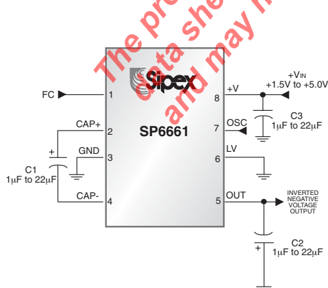
Figure 1: Voltage Inverter
