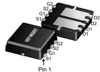
DFN3X3-8L (PowerPAK1212-8)
