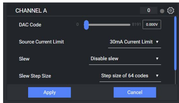
Figure 5. Channel Use Case Advanced Settings
