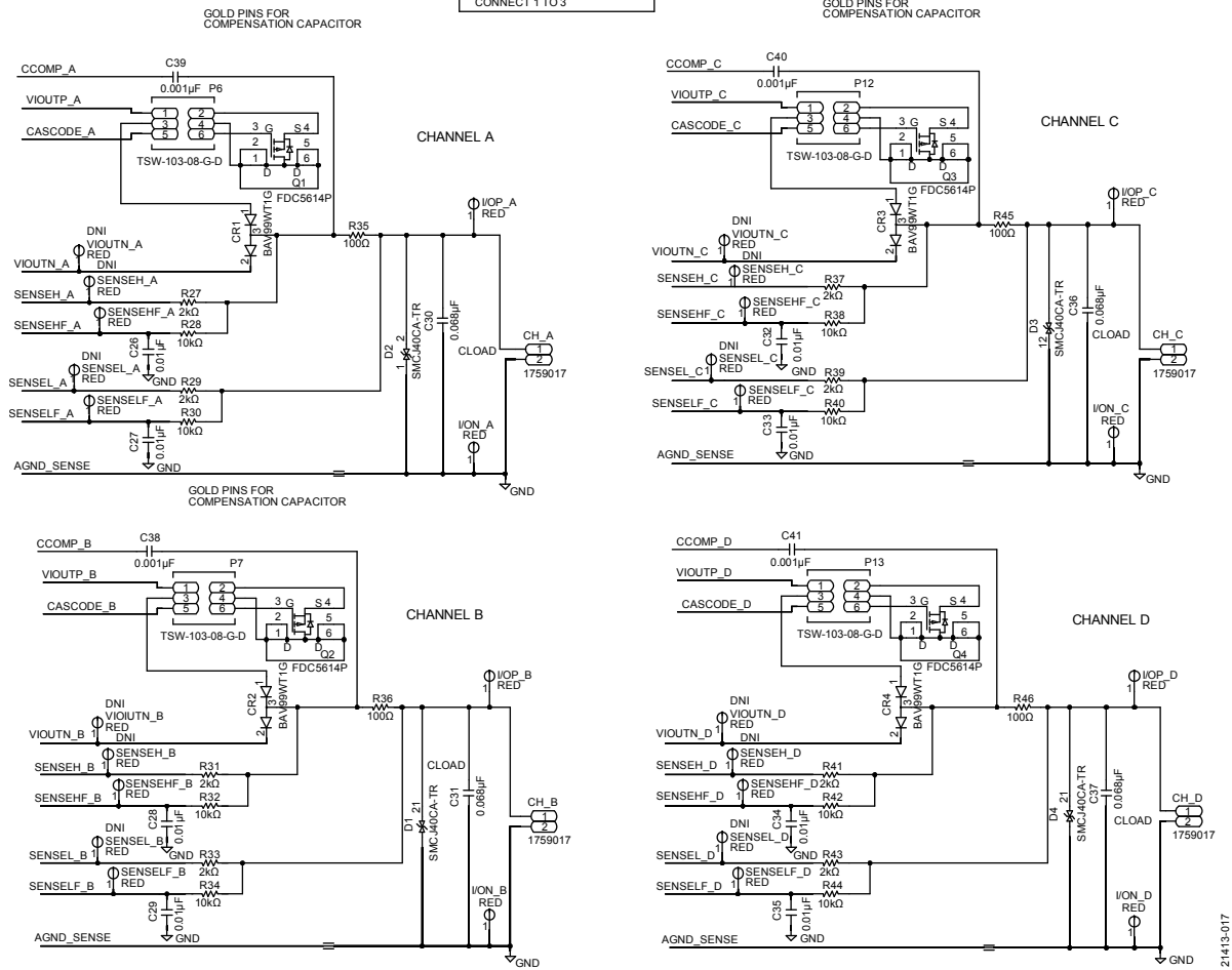
Figure 13. Channel Input/Output Circuitry Including Screw Terminals
