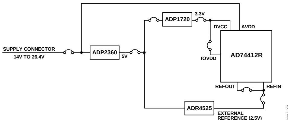
Figure 2. EV-AD74412RSDZ Simplified Power Diagram
