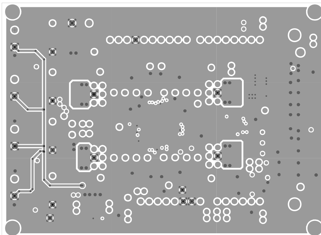
Figure 15. Layer 2, Ground Layer
