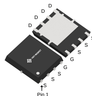
DFN5X6-8L (TDSO8-8-EP(5x6))
