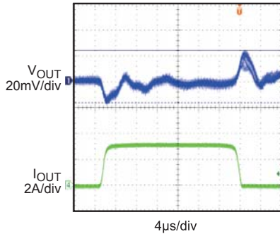
Transient Performance with @0.6 to 3.6A, 2.5A/μs
