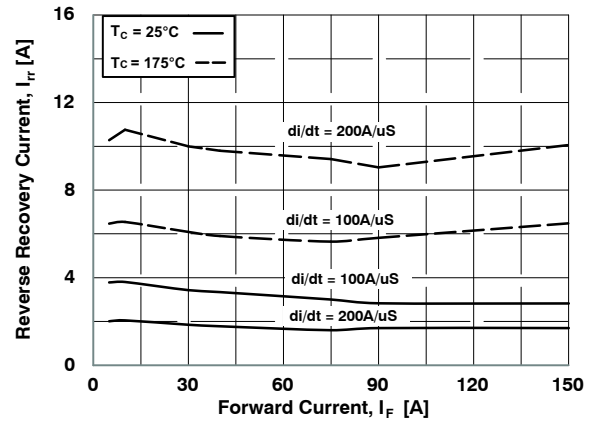
Figure 16. Reverse Recovery Current
