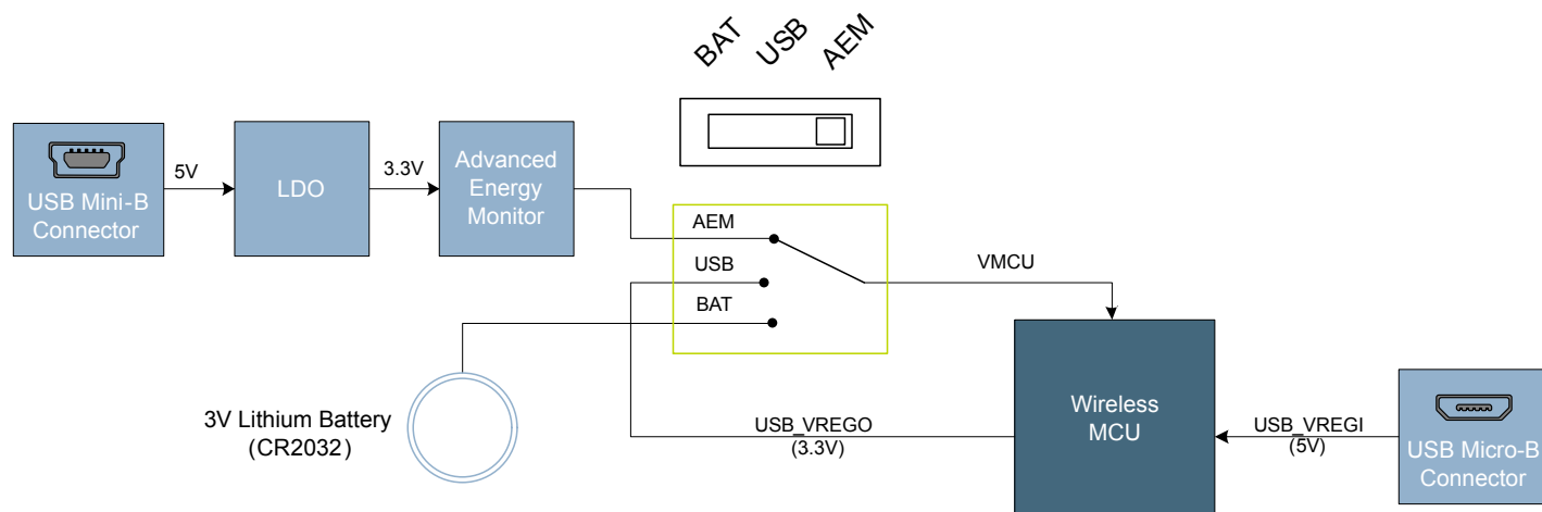
Figure 4.1. WSTK6200 Power Switch
