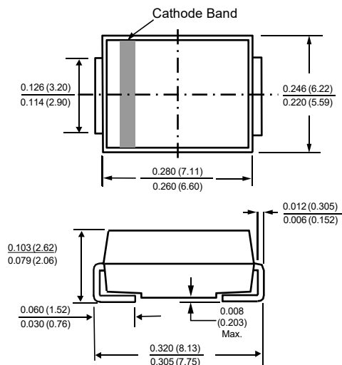
SMC (DO-214AB)
