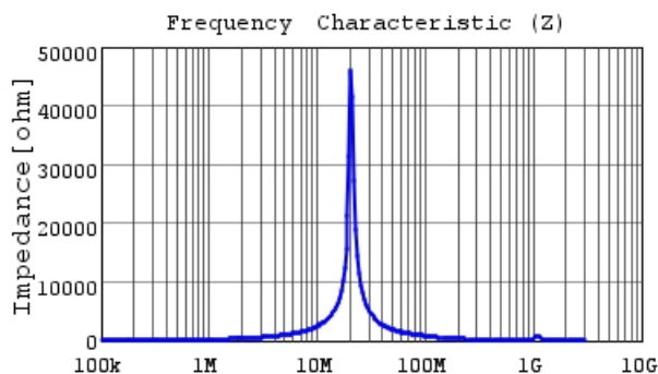
LQH43NZ330K03 |Z|
