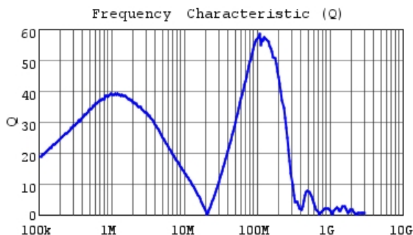
LQH43NZ330K03 Q
