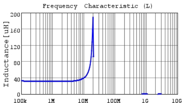
LQH43NZ330K03 L
