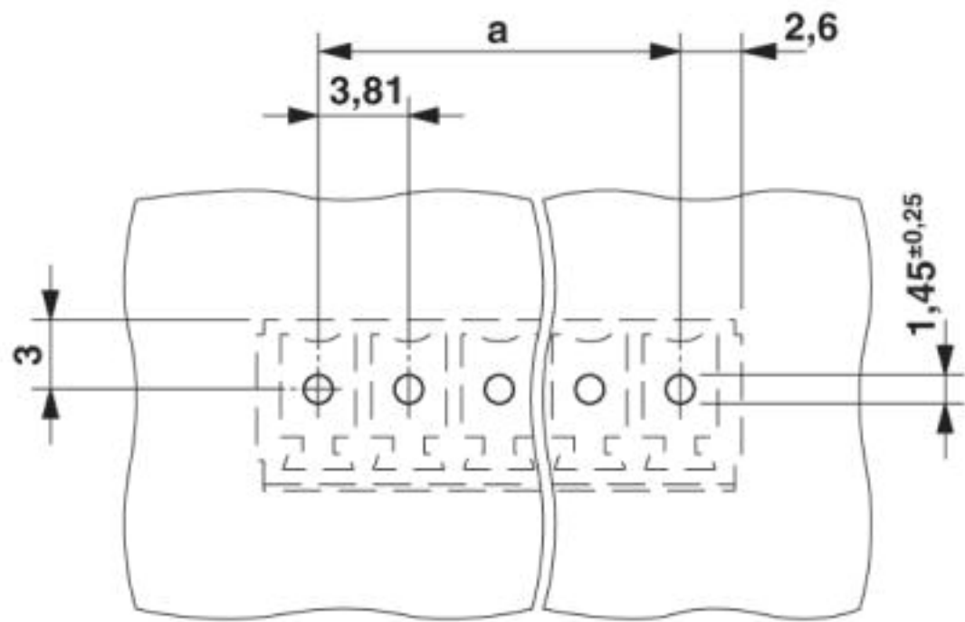
Drilling diagram
