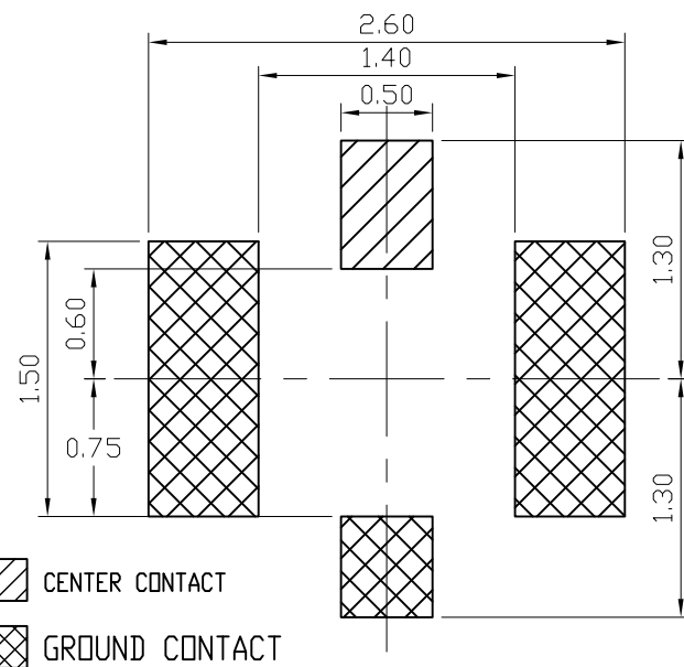
RECOMMENDED PCB LAYOUT (TOLERANCE: \pm 0.05 )
